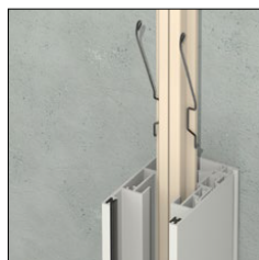
Compensation springs
