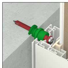
Adjustable spacers
