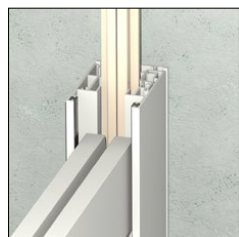
Front bar is connected to the guide rail
